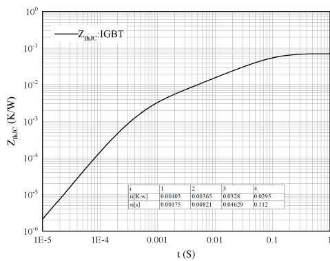
图 11. 瞬态热阻抗 IGBT 逆变器 Figure 11. Transient thermal impedance IGBT, Inverter Z_{thJC}=f(t)
