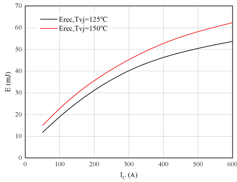
图 7. 开关损耗 二极管 Figure 7. Switching losses of Diode R_{Gon}=3.3\Omega, V_{CE}=900V
