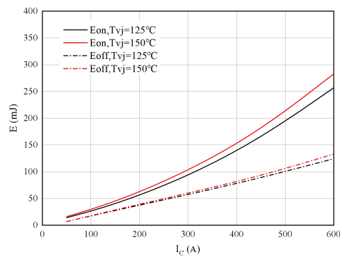
图 5. 开关损耗 逆变器 Figure 5. Switching losses of IGBT V_{GE}=\pm 15V, R_{Gon}=3.3\Omega, R_{Goff}=3.3\Omega, V_{CE}=900V
