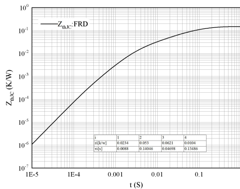
图 12. 瞬态热阻抗 FRD 逆变器 Figure 12. Transient thermal impedance FRD, Inverter Z_{thJC}=f(t)
