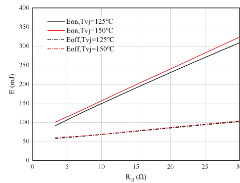
图 6. 开关损耗 逆变器 Figure 6. Switching losses of IGBT V_{GE}=\pm 15V, I_c=300A, V_{CE}=900V
